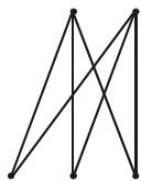
K_{2,3}
